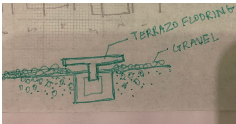
Flooring detail
