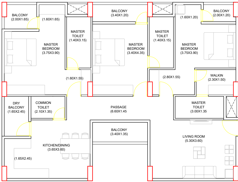
3BHK UNIT 1 - EVEN (155 SQ.M.)
