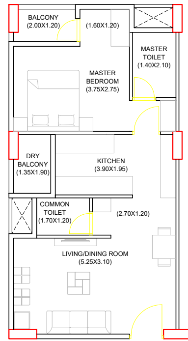
1BHK UNIT (58 SQ.M.)
