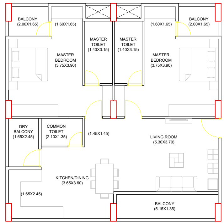
2BHK UNIT 1 (120 SQ.M.)
