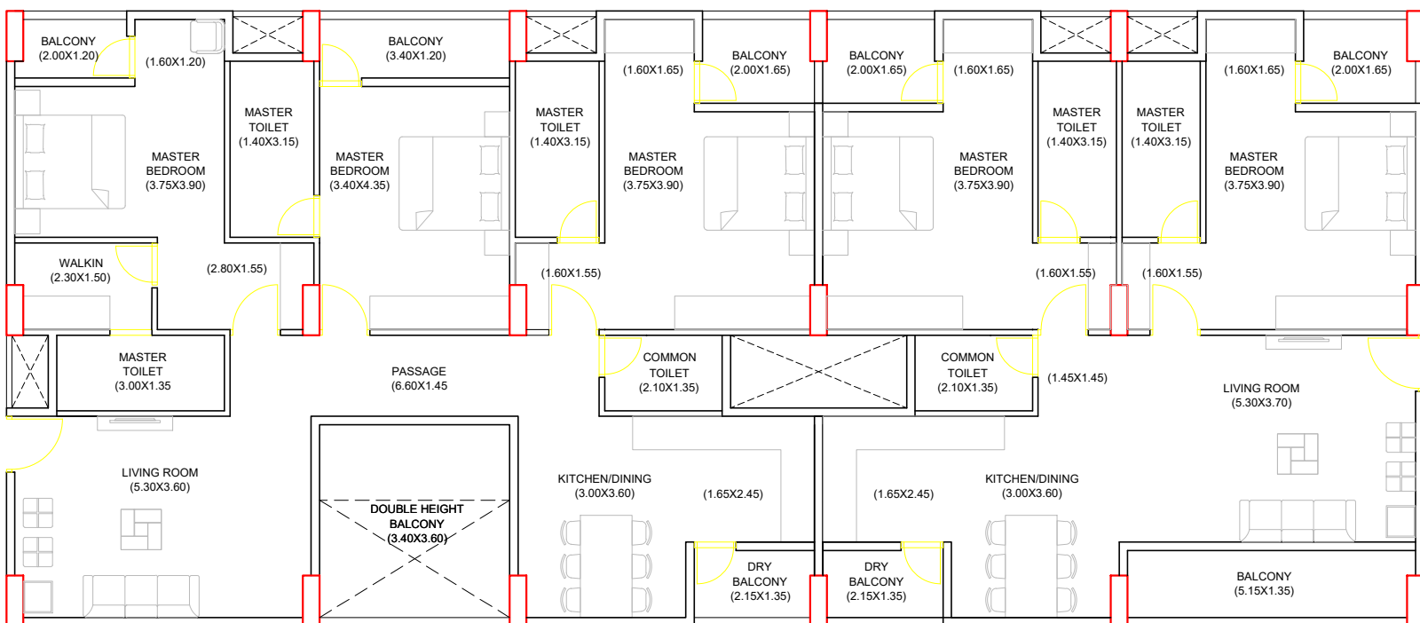
3BHK UNIT 2 (154 SQ.M.)
