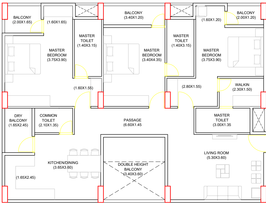
3BHK UNIT 1 - ODD (162 SQ.M.)
